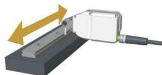
Linear geometry and parallelism measurement
